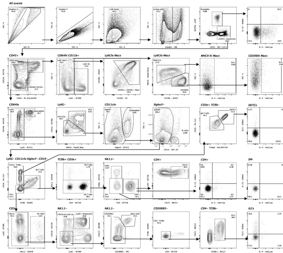
Figure 9. Gating strategy of the full 25 parameter staining panel of MC903 treated ear skin represented as contour plots gated in cascade. CD45 + leucocytes and YFP + basophils are gated from live single cells. CD64 + CD11b + macrophages were comprised of a Ly6C + inflammatory subset and two Ly6C lo subsets, MHCII hi or CD206 hi . From the CD64 lo population, Neutrophils are observed as CD11b + Ly6G + . In the Ly6G - population, dendritic cells were defined as MHCII + CD11c + . Eosinophils were gated as SiglecF + SSC hi cells from the CD11c lo subset, as were CD19 + B cells. Within the Ly6G - CD11c lo SiglecF - CD19 - population, TCRb + CD3 + T cells and CD3 + TCRb - T cells were identified. \alpha bT cells contained NK1.1 + NKTs, CD8 + , CD4 + and CD4 - CD8 - Double Negative (DN) T cells. The CD4 + subset further contained a population of CD25 + T cells. The TCRb - population could be divided in two subsets of \gamma \delta T cells, including a CD3/CD90.2/ \gamma \delta TCR hi Dendritic epidermal T cell population (DETC). CD3 negative subsets were gated as NK1.1 + NK cells, CD11b + Ly6C + inflammatory monocytes, CD11b - Ly6C - CD117 + CD200R3 + Mast cells, or Lineage - CD90.2 + CD25 + ILC2s. The expression of IL-4 and IL-13 by relevant immune cells was also analysed.
