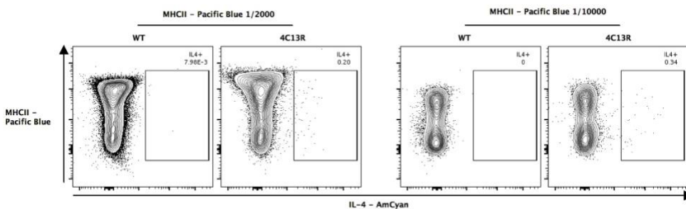
Figure 8. The spreading error of Pacific Blue MHCII in the AmCyan channel. Analysis of MC903 treated wild type (WT) ear skin revealed that the high expression of MHCII by CD45+ CD64+ CD11b+ macrophages was impeding the detection of IL4-AmCyan in the reporter mouse. Reducing the concentration of the MHCII-Pacific Blue antibody from the 1/2000 (left panel) to the 1/10000 dilution (right panel) did improve the detection of IL-4 by reducing the spreading error of Pacific Blue into the AmCyan channel.
