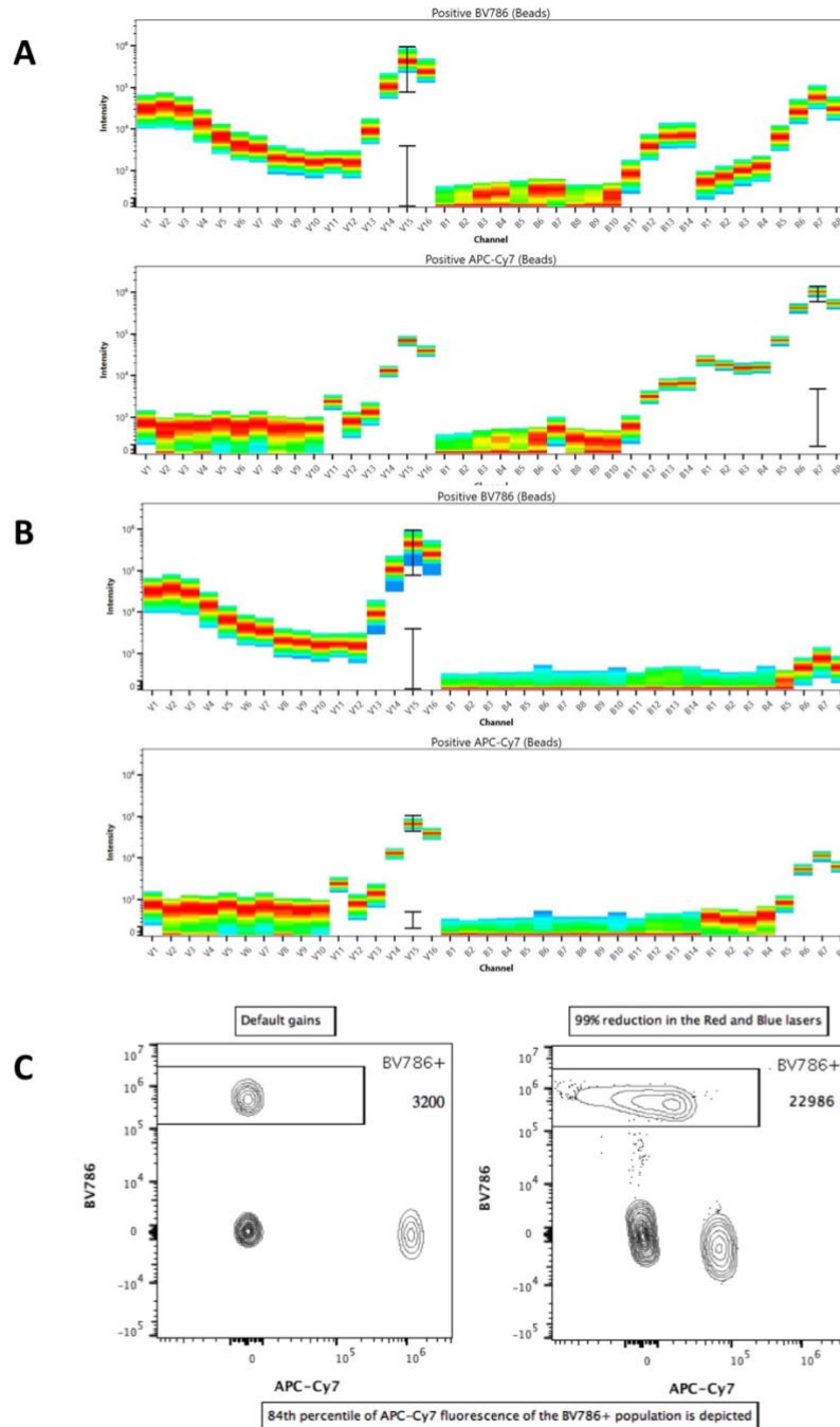
Figure 6. Compensation beads were stained with BV786 or APC-Cy7 conjugated antibodies and their spectral profile was acquired on an Aurora 3 laser system ( A ) using vendor established gains (“Cytek Assay Settings”) or ( B ) after a 99% reduction of the gains of all detectors associated with the red and blue lasers. Unmixing was performed for both data sets, and then single stained bead preparations were acquired in default or reduced gains conditions ( C ). The 84th percentile of the APC-Cy7 fluorescence detected on the BV786 + beads after spillover compensation (a measure of the SE^{16} ) is depicted on the dot plots. Note the width basis for data display needed to be further adjusted post gain reduction to produce the single BUV786 + population.
