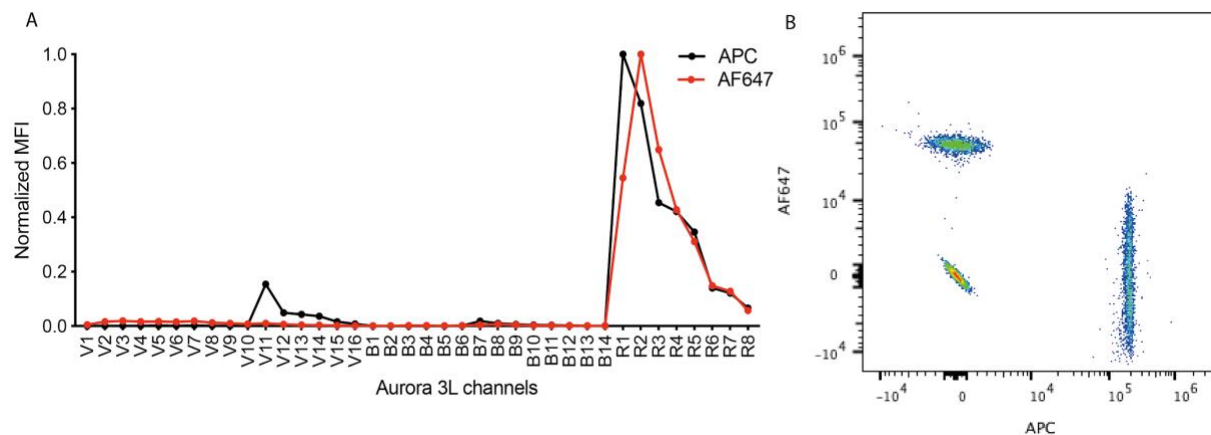
Figure 3. (A) Spectral pattern comparison (APC vs AF647); Note the stronger violet emission for APC compared with AF647 and differences in the peak emission profile (B) Dot plot showing that AF647 and APC stained beads can be discriminated by spectral flow cytometry, at the expense of significant spreading error.
